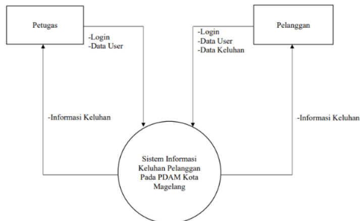
Gambar 2 Context Diagram
