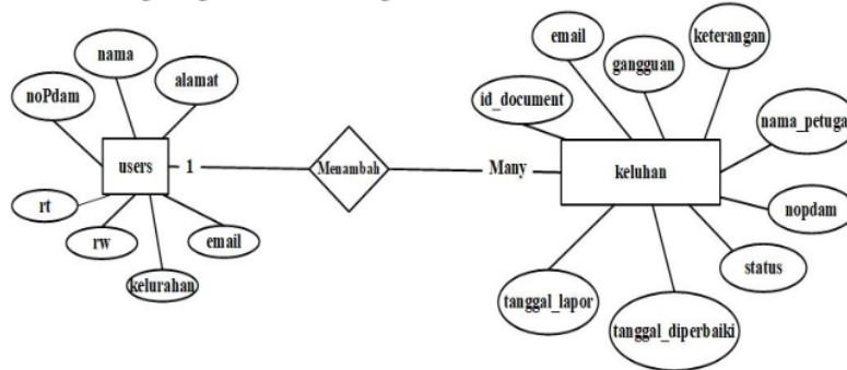
Gambar 3 ERD (Entitiy Relationship Diagram)
